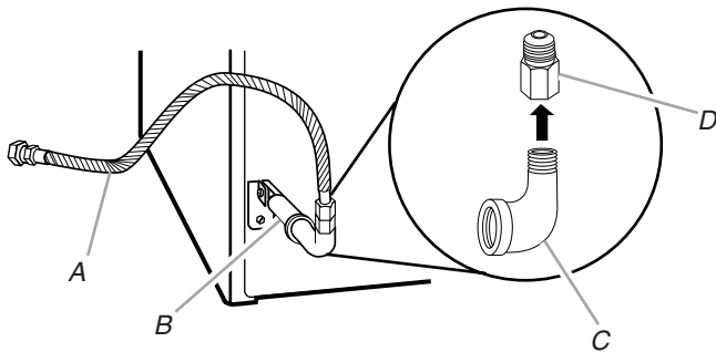
A. \frac{3}{8} " flexible gas connector B. \frac{3}{8} " dryer pipe C. \frac{3}{8} " to \frac{1}{2} " pipe elbow D. \frac{3}{8} " pipe-to-flare adapter fitting
